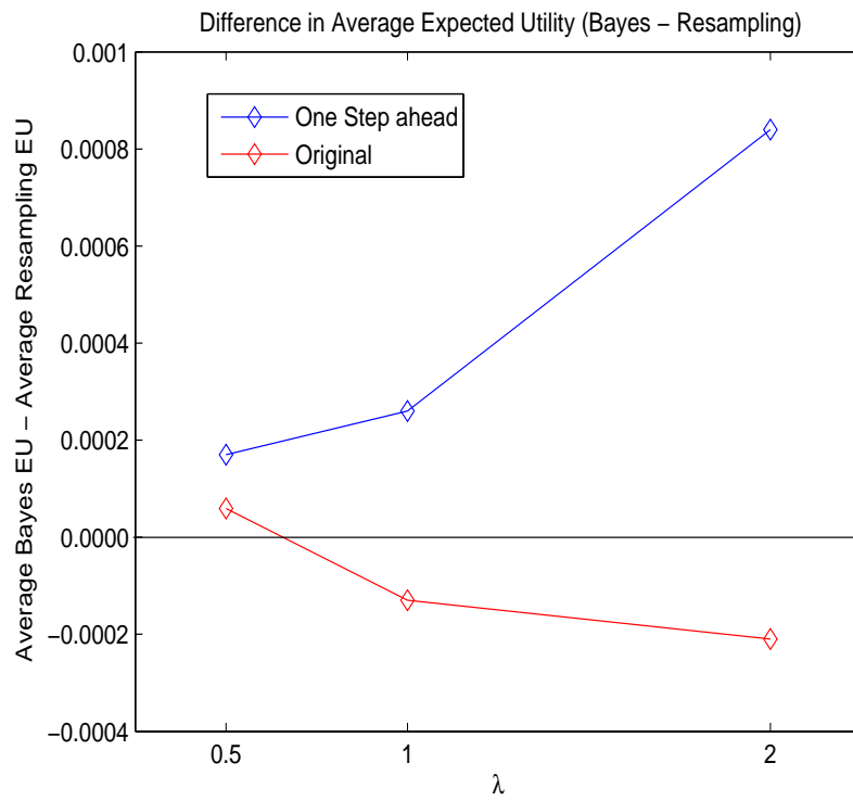
Figure 2: Difference in the average expected utility (Bayes - Resampling) as a function of risk aversion (or \lambda ). Results are for the original game and for the new game (or one-step ahead game).
